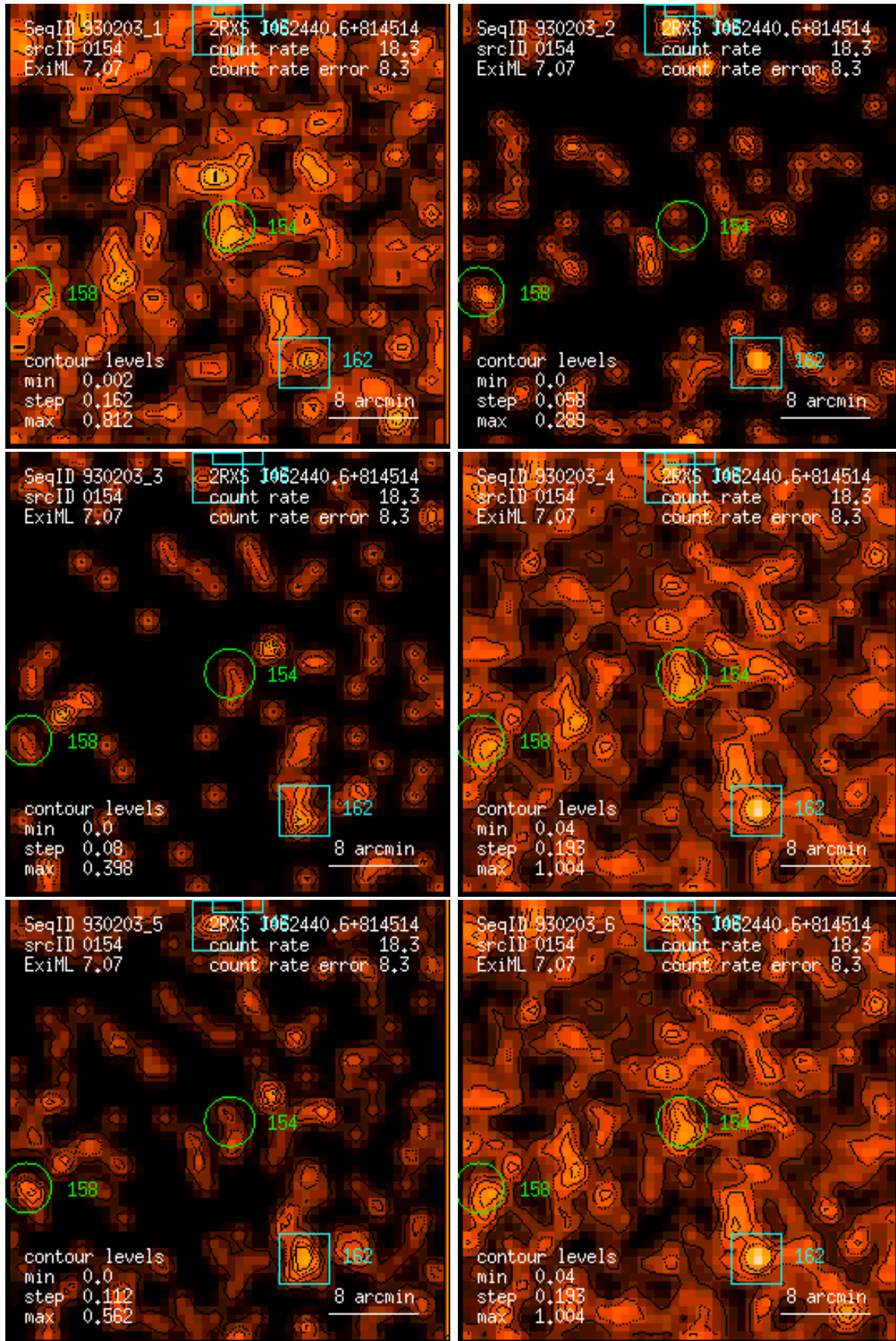
Figure 154: RASS 930203: detection 0154: band rate images, Gaussian filter: (1) PSPC channels 11 – 41, (2) 52 – 90, (3) 91 – 201, (4) 11 – 235, (5) 52 – 201, (6) 11 – 201. Broad band rates in counts/ks. Band rate contour levels in counts/ks/arcmin 2 .
