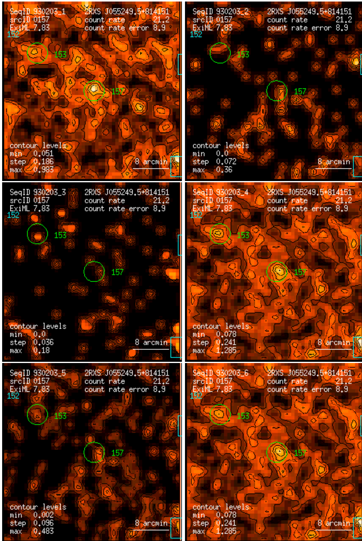
Figure 157: RASS 930203: detection 0157: band rate images, Gaussian filter: (1) PSPC channels 11 – 41, (2) 52 – 90, (3) 91 – 201, (4) 11 – 235, (5) 52 – 201, (6) 11 – 201. Broad band rates in counts/ks. Band rate contour levels in counts/ks/arcmin 2 .
