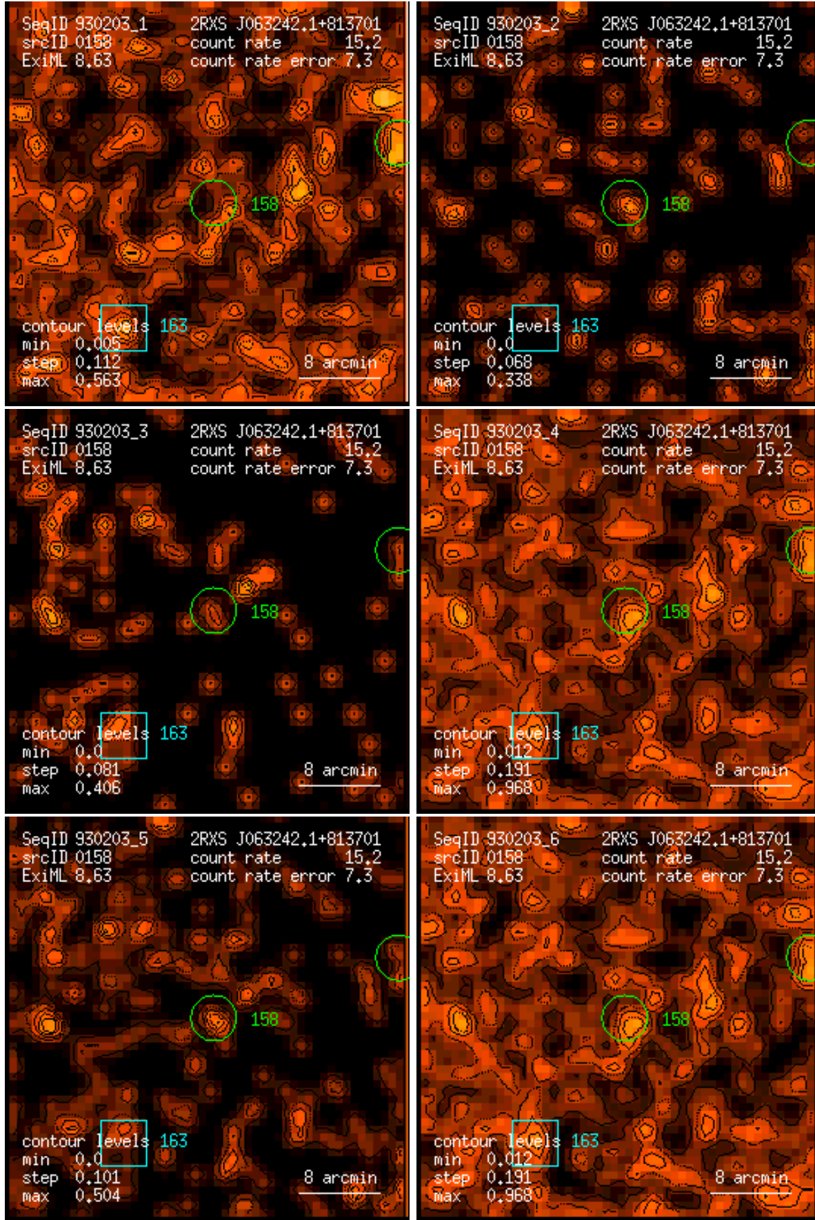
Figure 158: RASS 930203: detection 0158: band rate images, Gaussian filter: (1) PSPC channels 11 – 41, (2) 52 – 90, (3) 91 – 201, (4) 11 – 235, (5) 52 – 201, (6) 11 – 201. Broad band rates in counts/ks. Band rate contour levels in counts/ks/arcmin 2 .
