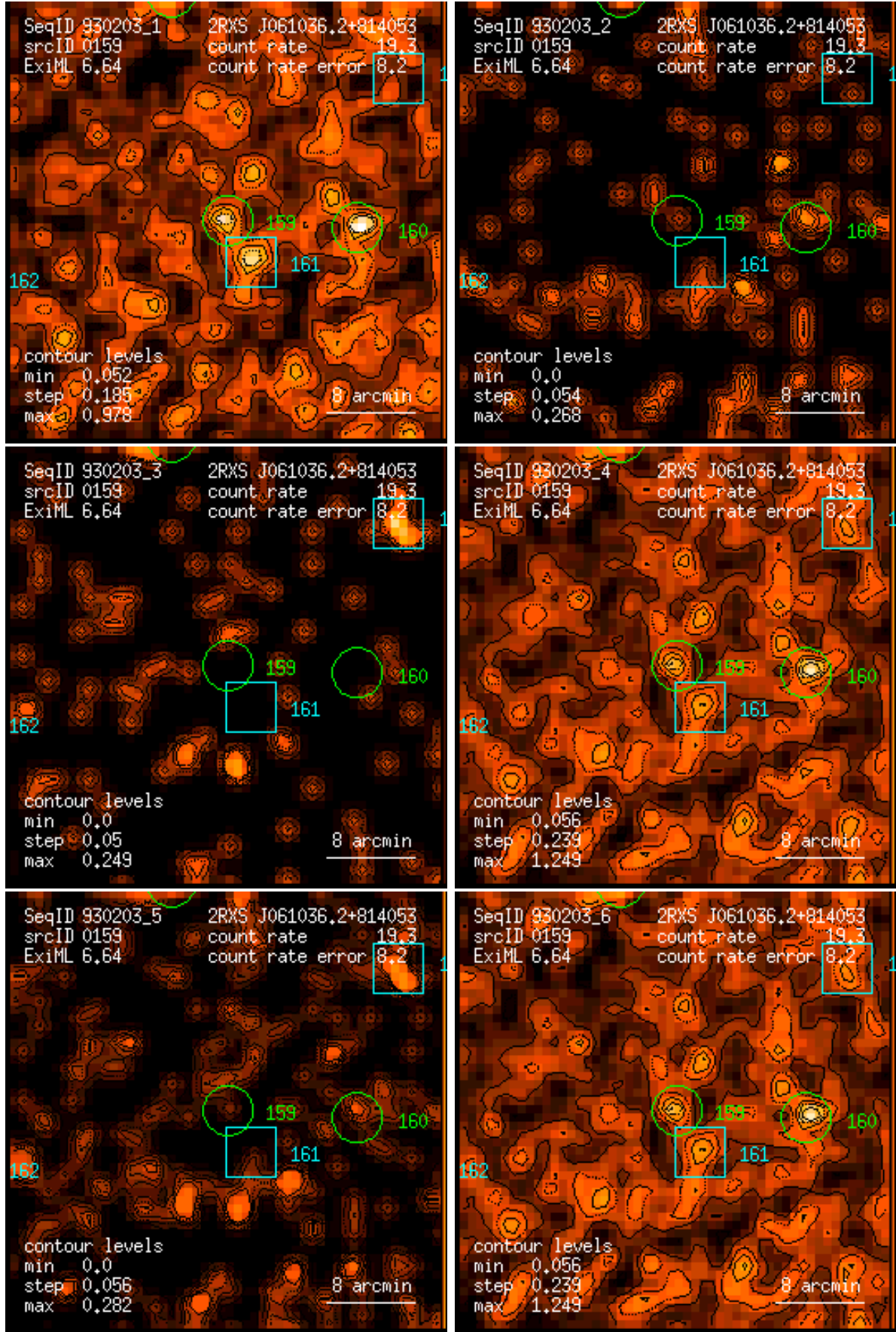
Figure 159: RASS 930203: detection 0159: band rate images, Gaussian filter: (1) PSPC channels 11 – 41, (2) 52 – 90, (3) 91 – 201, (4) 11 – 235, (5) 52 – 201, (6) 11 – 201. Broad band rates in counts/ks. Band rate contour levels in counts/ks/arcmin 2 .
