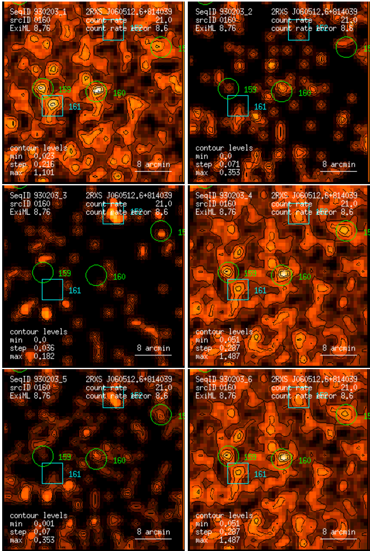
Figure 160: RASS 930203: detection 0160: band rate images, Gaussian filter: (1) PSPC channels 11 – 41, (2) 52 – 90, (3) 91 – 201, (4) 11 – 235, (5) 52 – 201, (6) 11 – 201. Broad band rates in counts/ks. Band rate contour levels in counts/ks/arcmin 2 .
