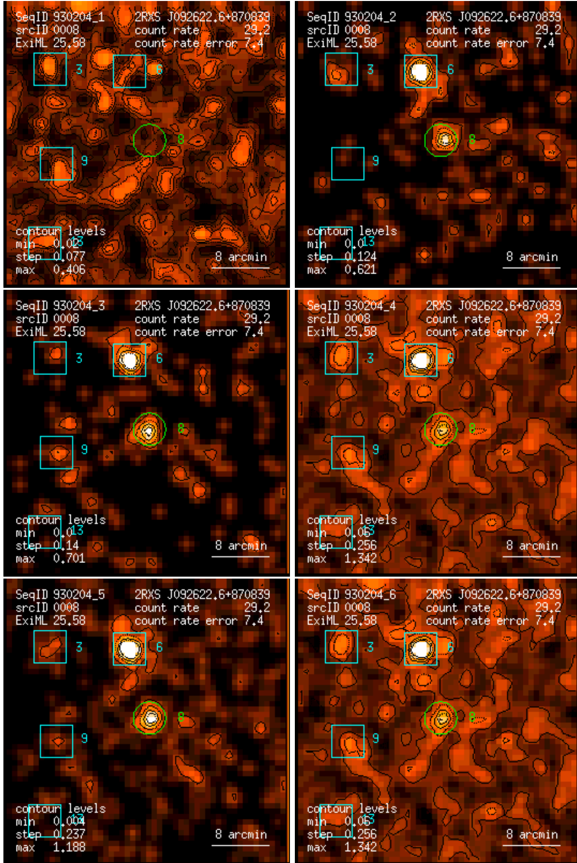
Figure 8: RASS 930204: detection 0008: band rate images, Gaussian filter: (1) PSPC channels 11 – 41, (2) 52 – 90, (3) 91 – 201, (4) 11 – 235, (5) 52 – 201, (6) 11 – 201. Broad band rates in counts/ks. Band rate contour levels in counts/ks/arcmin 2 .
