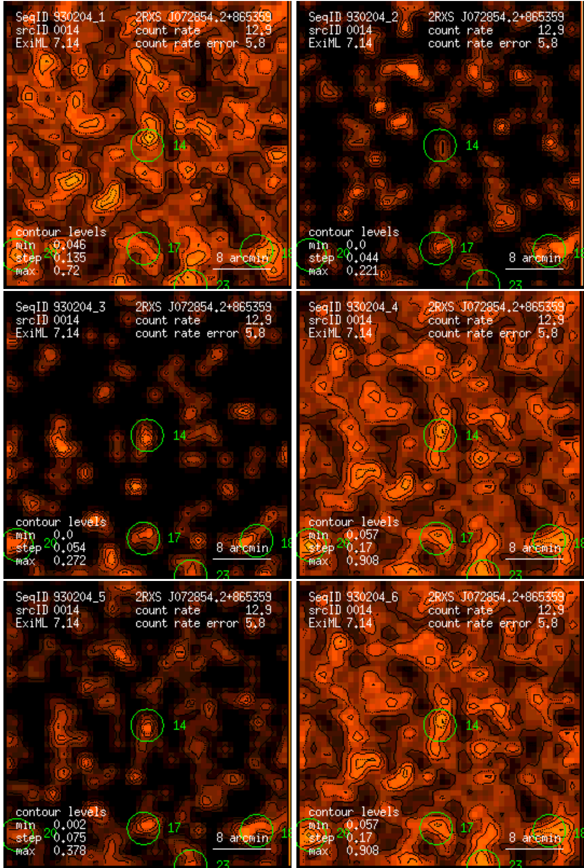
Figure 14: RASS 930204: detection 0014: band rate images, Gaussian filter: (1) PSPC channels 11 – 41, (2) 52 – 90, (3) 91 – 201, (4) 11 – 235, (5) 52 – 201, (6) 11 – 201. Broad band rates in counts/ks. Band rate contour levels in counts/ks/arcmin 2 .
