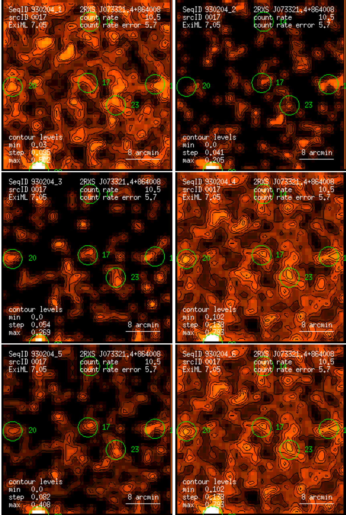
Figure 17: RASS 930204: detection 0017: band rate images, Gaussian filter: (1) PSPC channels 11 – 41, (2) 52 – 90, (3) 91 – 201, (4) 11 – 235, (5) 52 – 201, (6) 11 – 201. Broad band rates in counts/ks. Band rate contour levels in counts/ks/arcmin 2 .
