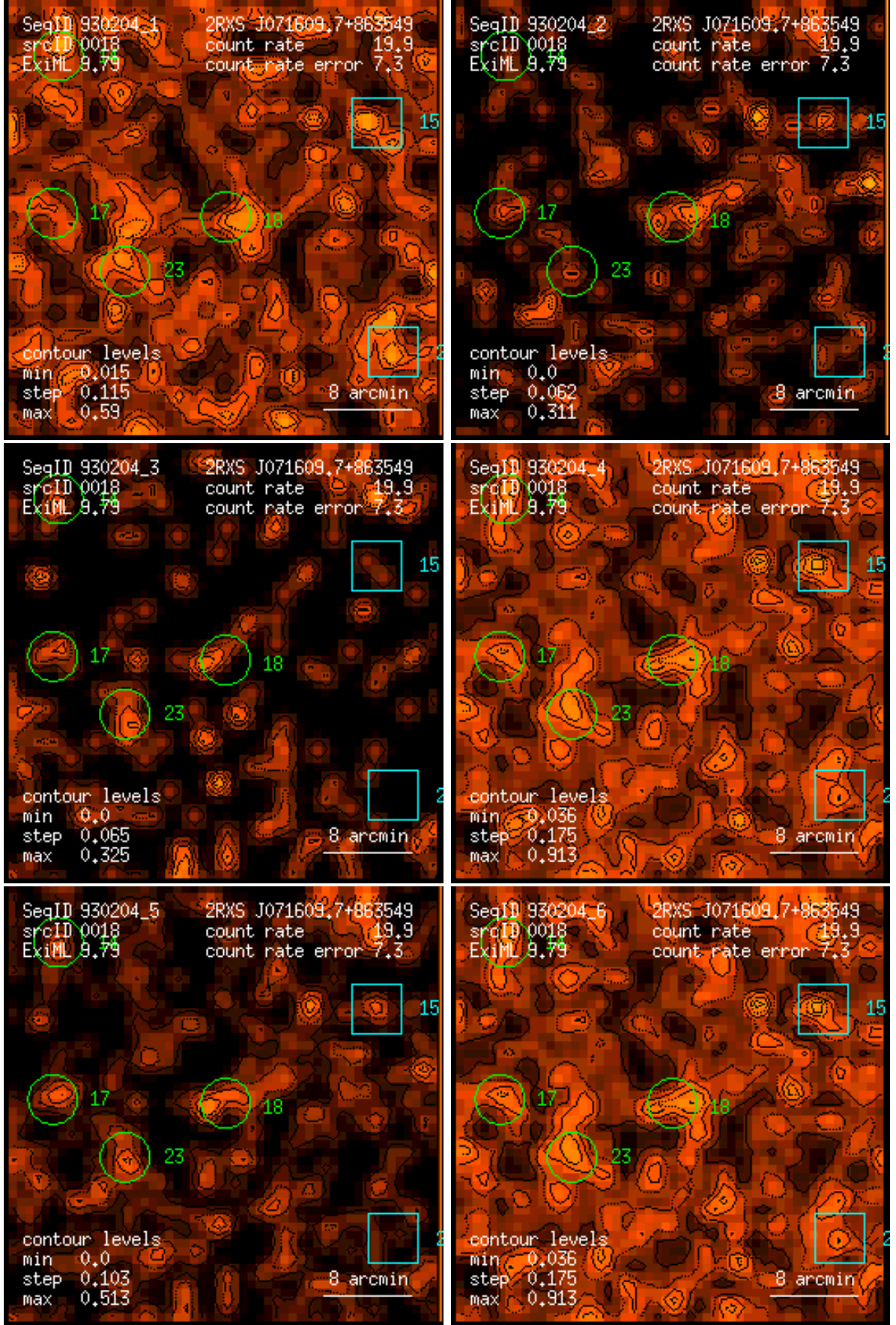
Figure 18: RASS 930204: detection 0018: band rate images, Gaussian filter: (1) PSPC channels 11 – 41, (2) 52 – 90, (3) 91 – 201, (4) 11 – 235, (5) 52 – 201, (6) 11 – 201. Broad band rates in counts/ks. Band rate contour levels in counts/ks/arcmin 2 .
