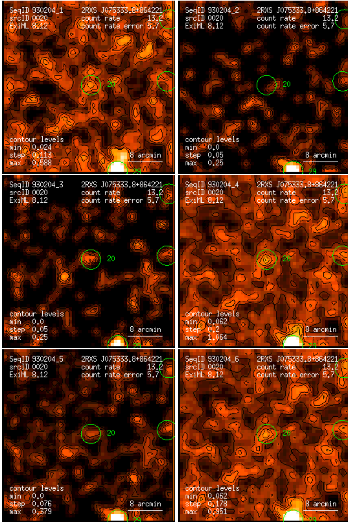
Figure 20: RASS 930204: detection 0020: band rate images, Gaussian filter: (1) PSPC channels 11 – 41, (2) 52 – 90, (3) 91 – 201, (4) 11 – 235, (5) 52 – 201, (6) 11 – 201. Broad band rates in counts/ks. Band rate contour levels in counts/ks/arcmin 2 .
