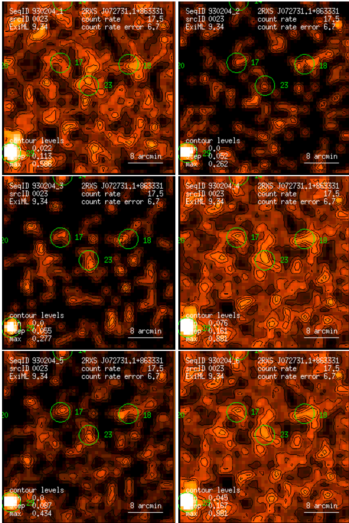
Figure 23: RASS 930204: detection 0023: band rate images, Gaussian filter: (1) PSPC channels 11 – 41, (2) 52 – 90, (3) 91 – 201, (4) 11 – 235, (5) 52 – 201, (6) 11 – 201. Broad band rates in counts/ks. Band rate contour levels in counts/ks/arcmin 2 .
