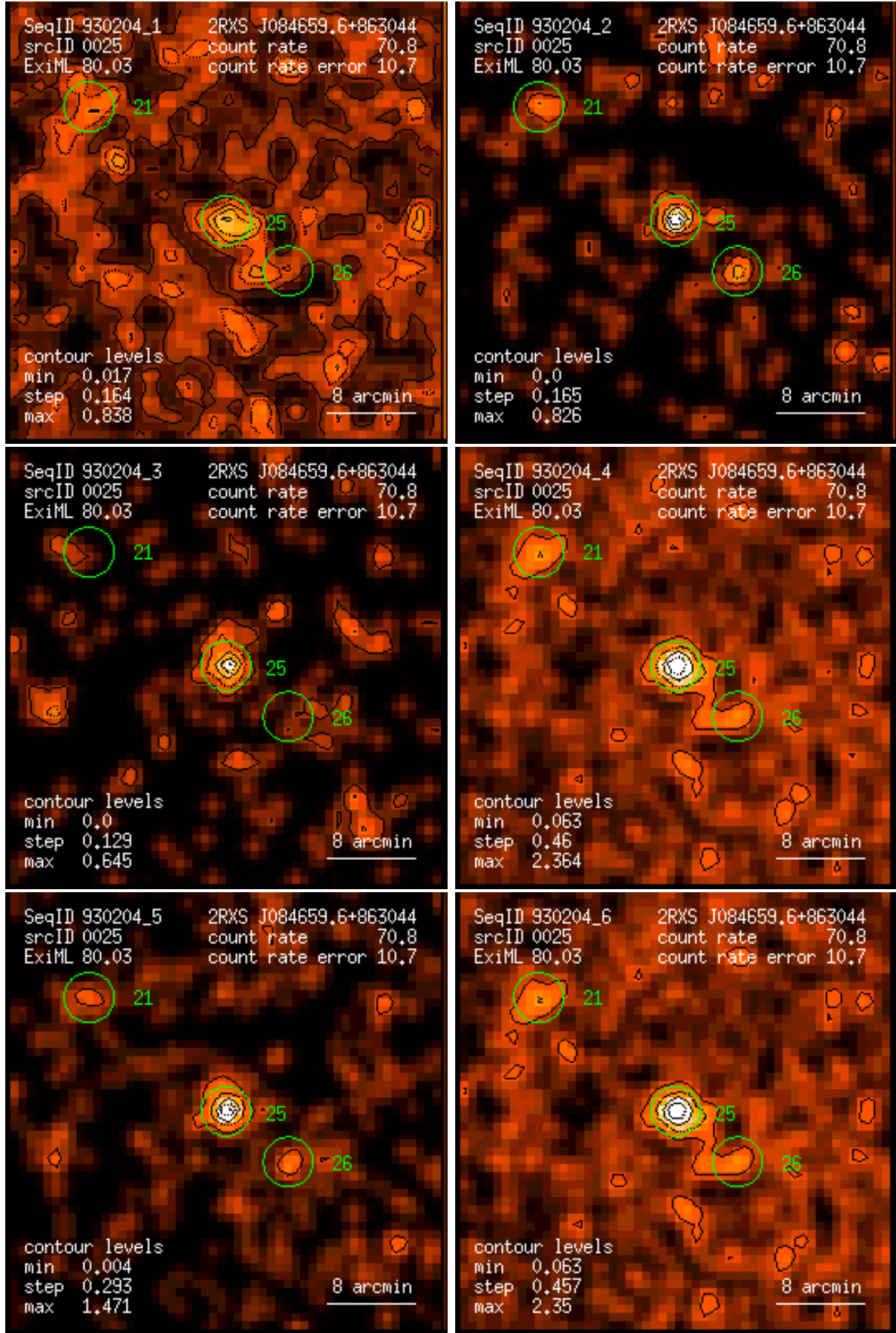
Figure 25: RASS 930204: detection 0025: band rate images, Gaussian filter: (1) PSPC channels 11 – 41, (2) 52 – 90, (3) 91 – 201, (4) 11 – 235, (5) 52 – 201, (6) 11 – 201. Broad band rates in counts/ks. Band rate contour levels in counts/ks/arcmin 2 .
