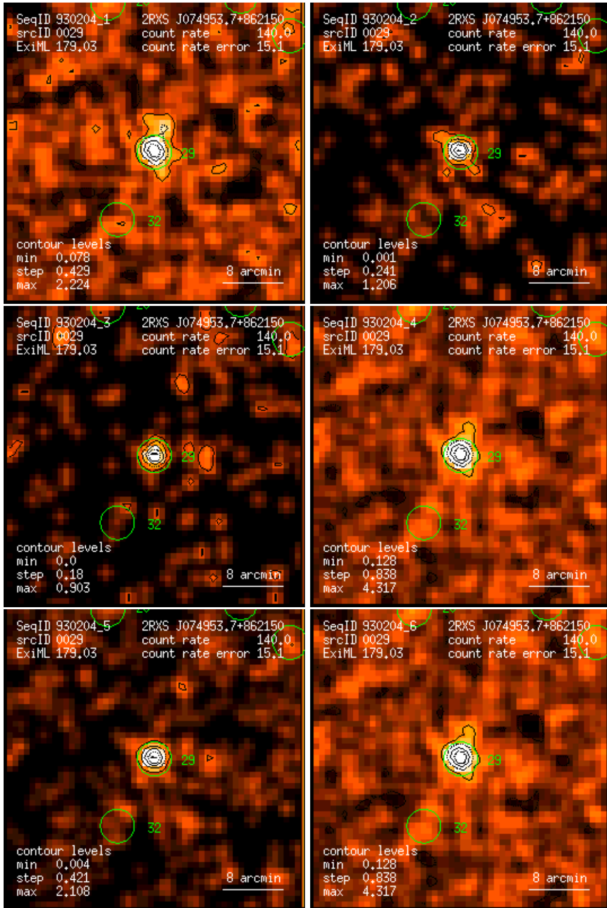
Figure 29: RASS 930204: detection 0029: band rate images, Gaussian filter: (1) PSPC channels 11 – 41, (2) 52 – 90, (3) 91 – 201, (4) 11 – 235, (5) 52 – 201, (6) 11 – 201. Broad band rates in counts/ks. Band rate contour levels in counts/ks/arcmin 2 .
