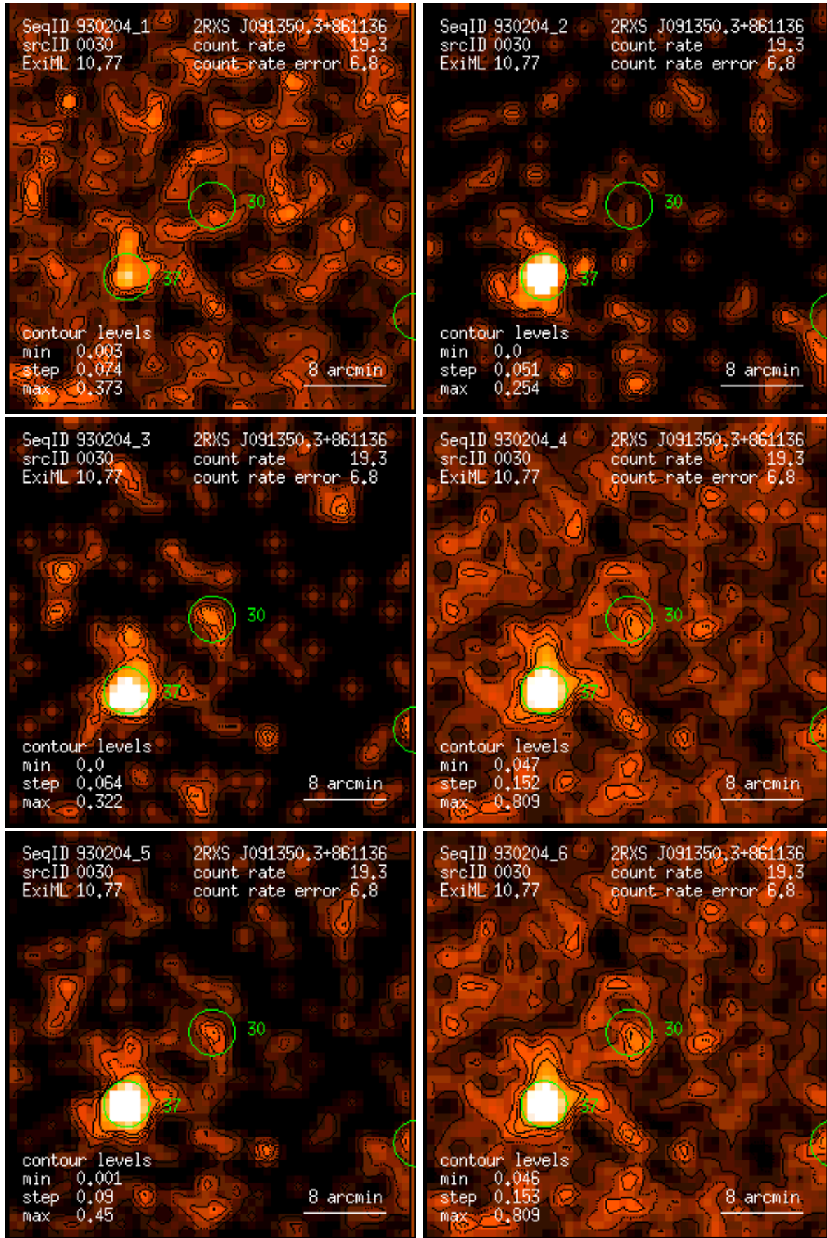
Figure 30: RASS 930204: detection 0030: band rate images, Gaussian filter: (1) PSPC channels 11 – 41, (2) 52 – 90, (3) 91 – 201, (4) 11 – 235, (5) 52 – 201, (6) 11 – 201. Broad band rates in counts/ks. Band rate contour levels in counts/ks/arcmin 2 .
