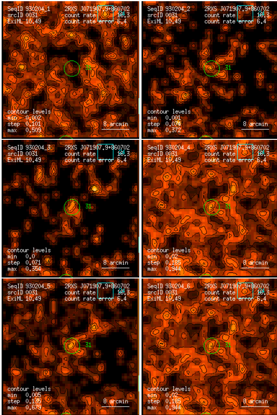
Figure 31: RASS 930204: detection 0031: band rate images, Gaussian filter: (1) PSPC channels 11 – 41, (2) 52 – 90, (3) 91 – 201, (4) 11 – 235, (5) 52 – 201, (6) 11 – 201. Broad band rates in counts/ks. Band rate contour levels in counts/ks/arcmin 2 .
