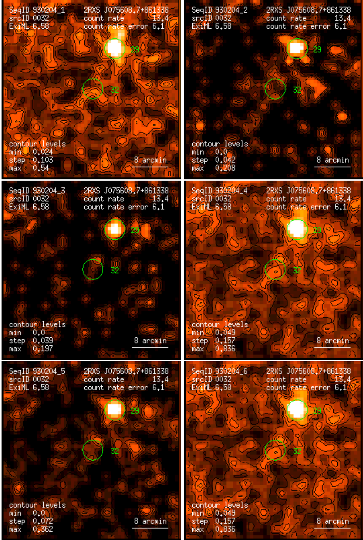
Figure 32: RASS 930204: detection 0032: band rate images, Gaussian filter: (1) PSPC channels 11 – 41, (2) 52 – 90, (3) 91 – 201, (4) 11 – 235, (5) 52 – 201, (6) 11 – 201. Broad band rates in counts/ks. Band rate contour levels in counts/ks/arcmin 2 .
