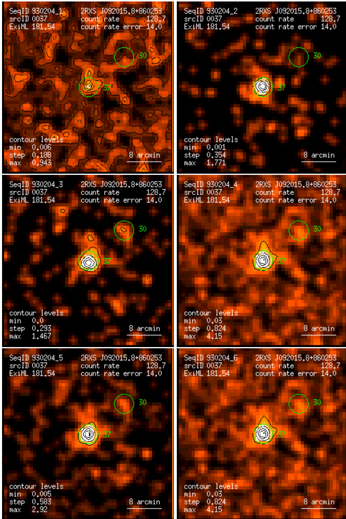
Figure 37: RASS 930204: detection 0037: band rate images, Gaussian filter: (1) PSPC channels 11 – 41, (2) 52 – 90, (3) 91 – 201, (4) 11 – 235, (5) 52 – 201, (6) 11 – 201. Broad band rates in counts/ks. Band rate contour levels in counts/ks/arcmin 2 .
