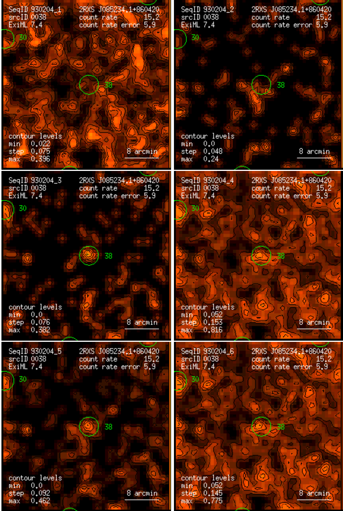
Figure 38: RASS 930204: detection 0038: band rate images, Gaussian filter: (1) PSPC channels 11 – 41, (2) 52 – 90, (3) 91 – 201, (4) 11 – 235, (5) 52 – 201, (6) 11 – 201. Broad band rates in counts/ks. Band rate contour levels in counts/ks/arcmin 2 .
