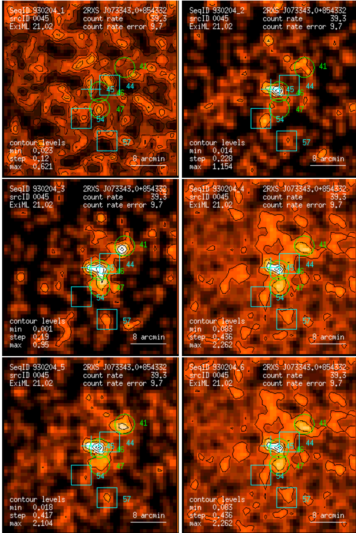
Figure 45: RASS 930204: detection 0045: band rate images, Gaussian filter: (1) PSPC channels 11 – 41, (2) 52 – 90, (3) 91 – 201, (4) 11 – 235, (5) 52 – 201, (6) 11 – 201. Broad band rates in counts/ks. Band rate contour levels in counts/ks/arcmin 2 .
