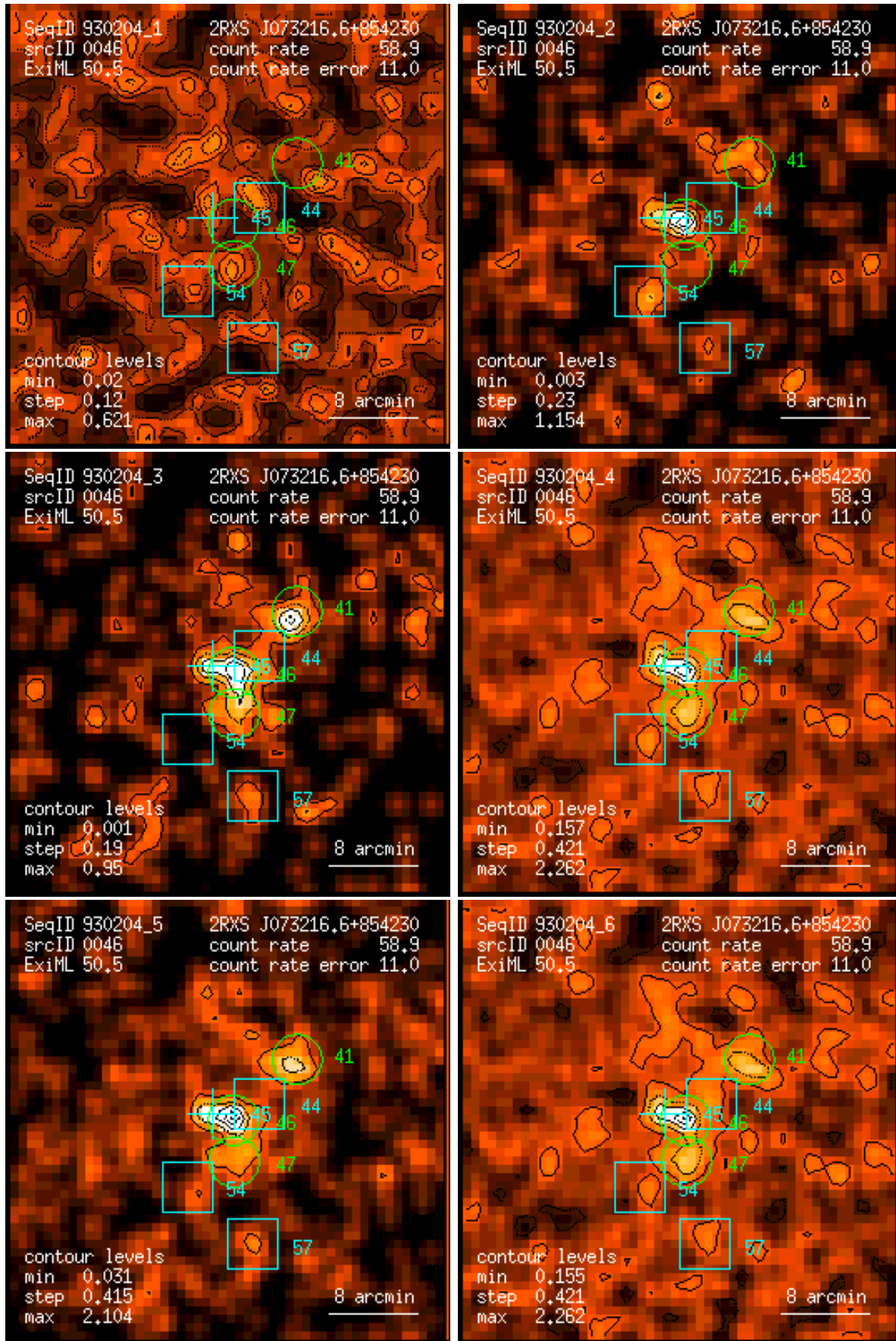
Figure 46: RASS 930204: detection 0046: band rate images, Gaussian filter: (1) PSPC channels 11 – 41, (2) 52 – 90, (3) 91 – 201, (4) 11 – 235, (5) 52 – 201, (6) 11 – 201. Broad band rates in counts/ks. Band rate contour levels in counts/ks/arcmin 2 .
