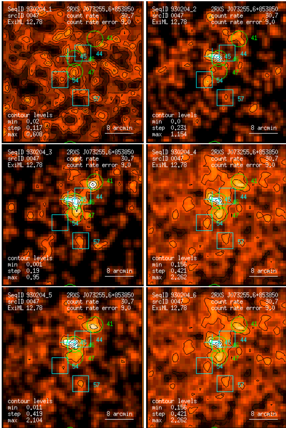
Figure 47: RASS 930204: detection 0047: band rate images, Gaussian filter: (1) PSPC channels 11 – 41, (2) 52 – 90, (3) 91 – 201, (4) 11 – 235, (5) 52 – 201, (6) 11 – 201. Broad band rates in counts/ks. Band rate contour levels in counts/ks/arcmin 2 .
