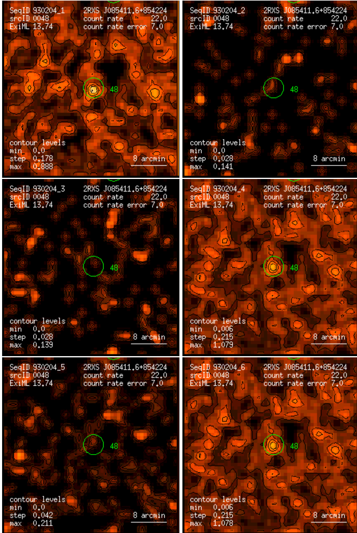
Figure 48: RASS 930204: detection 0048: band rate images, Gaussian filter: (1) PSPC channels 11 – 41, (2) 52 – 90, (3) 91 – 201, (4) 11 – 235, (5) 52 – 201, (6) 11 – 201. Broad band rates in counts/ks. Band rate contour levels in counts/ks/arcmin 2 .
