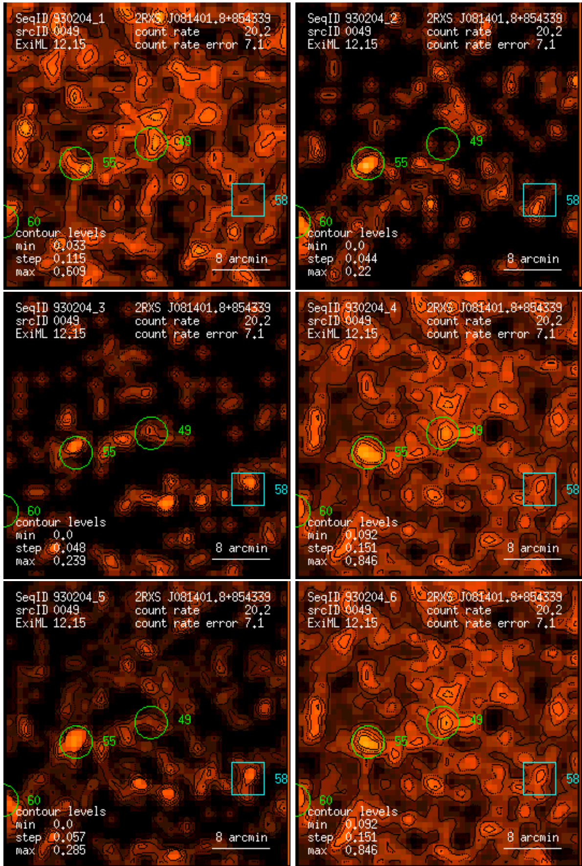
Figure 49: RASS 930204: detection 0049: band rate images, Gaussian filter: (1) PSPC channels 11 – 41, (2) 52 – 90, (3) 91 – 201, (4) 11 – 235, (5) 52 – 201, (6) 11 – 201. Broad band rates in counts/ks. Band rate contour levels in counts/ks/arcmin 2 .
