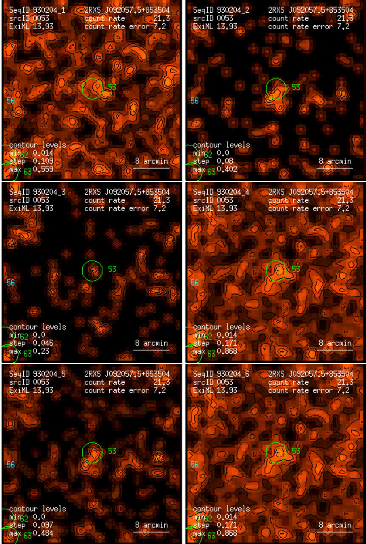
Figure 53: RASS 930204: detection 0053: band rate images, Gaussian filter: (1) PSPC channels 11 – 41, (2) 52 – 90, (3) 91 – 201, (4) 11 – 235, (5) 52 – 201, (6) 11 – 201. Broad band rates in counts/ks. Band rate contour levels in counts/ks/arcmin 2 .
