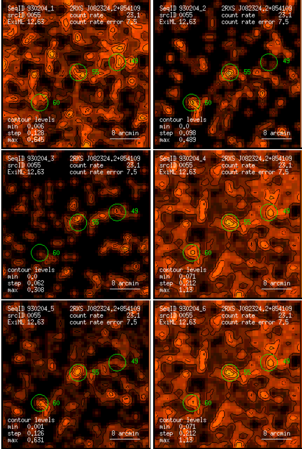
Figure 55: RASS 930204: detection 0055: band rate images, Gaussian filter: (1) PSPC channels 11 – 41, (2) 52 – 90, (3) 91 – 201, (4) 11 – 235, (5) 52 – 201, (6) 11 – 201. Broad band rates in counts/ks. Band rate contour levels in counts/ks/arcmin 2 .
