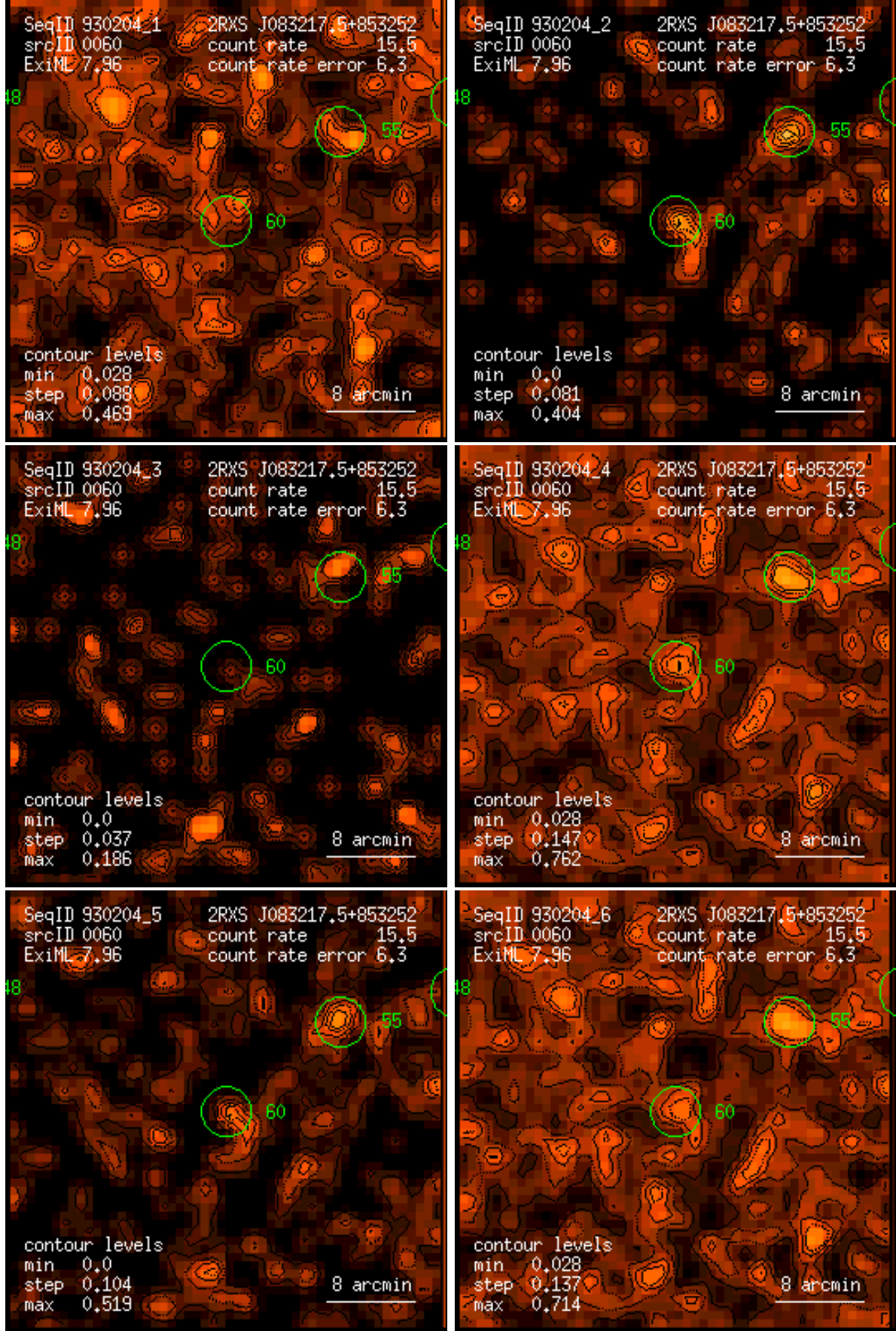
Figure 60: RASS 930204: detection 0060: band rate images, Gaussian filter: (1) PSPC channels 11 – 41, (2) 52 – 90, (3) 91 – 201, (4) 11 – 235, (5) 52 – 201, (6) 11 – 201. Broad band rates in counts/ks. Band rate contour levels in counts/ks/arcmin 2 .
