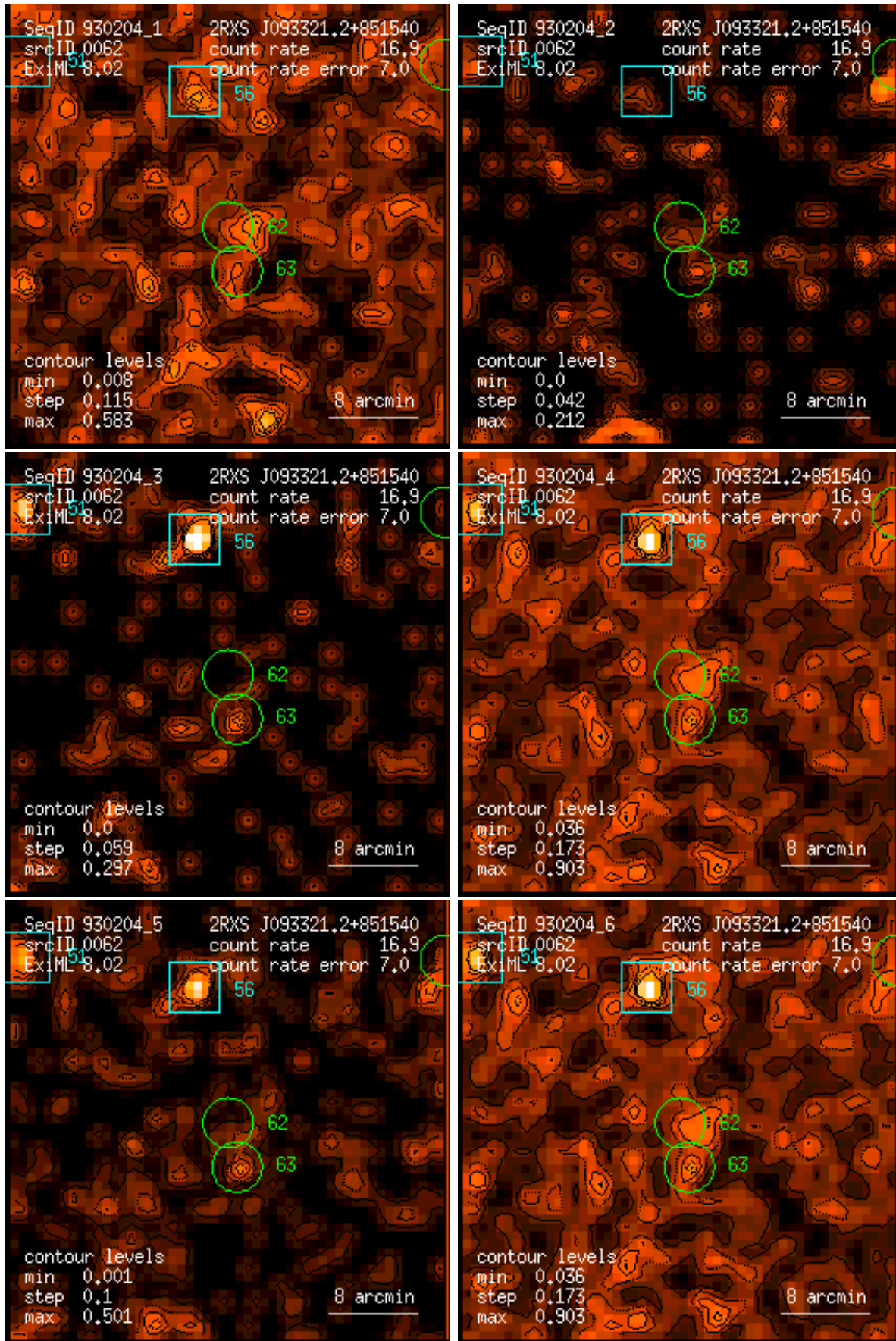
Figure 62: RASS 930204: detection 0062: band rate images, Gaussian filter: (1) PSPC channels 11 – 41, (2) 52 – 90, (3) 91 – 201, (4) 11 – 235, (5) 52 – 201, (6) 11 – 201. Broad band rates in counts/ks. Band rate contour levels in counts/ks/arcmin 2 .
