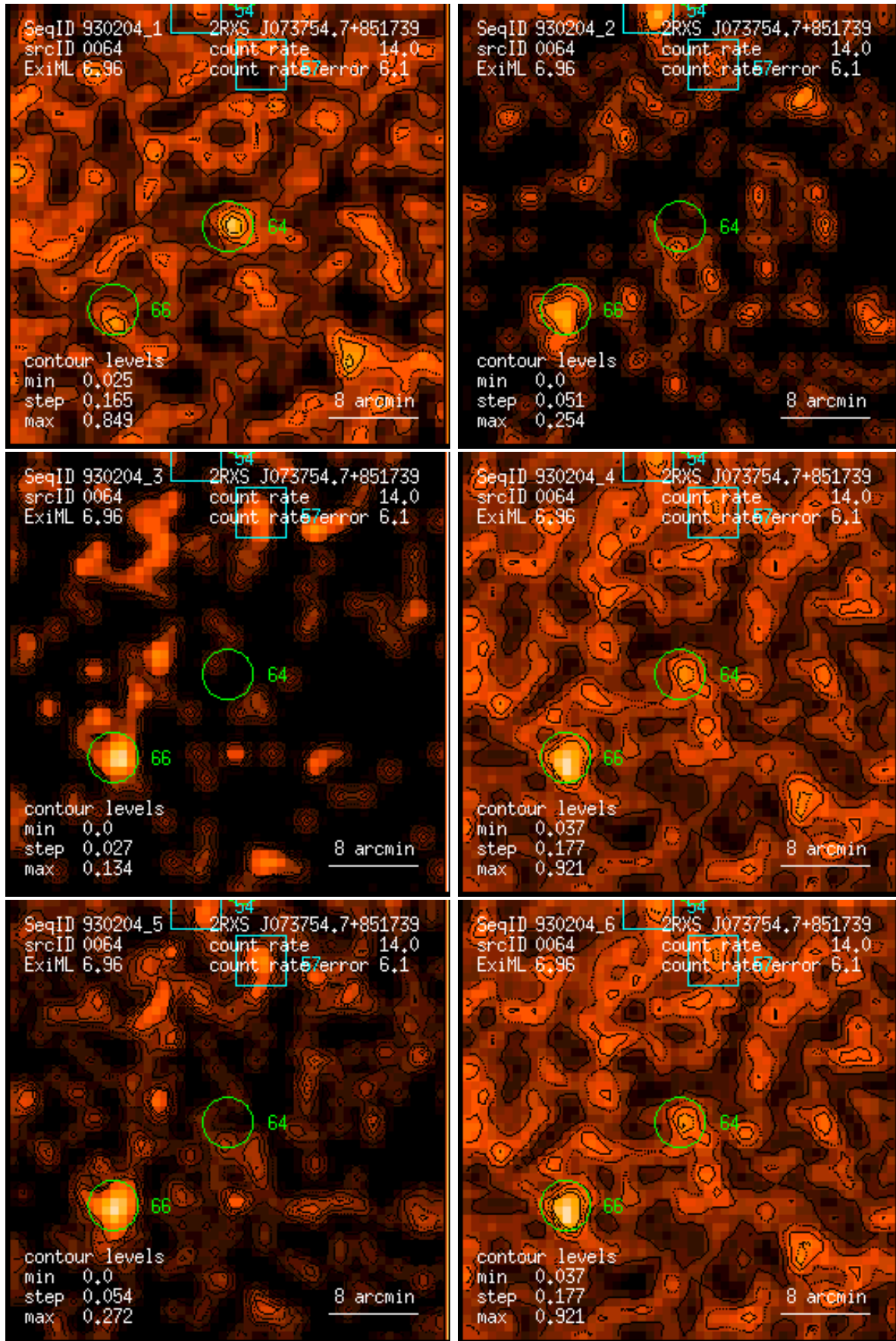
Figure 64: RASS 930204: detection 0064: band rate images, Gaussian filter: (1) PSPC channels 11 – 41, (2) 52 – 90, (3) 91 – 201, (4) 11 – 235, (5) 52 – 201, (6) 11 – 201. Broad band rates in counts/ks. Band rate contour levels in counts/ks/arcmin 2 .
