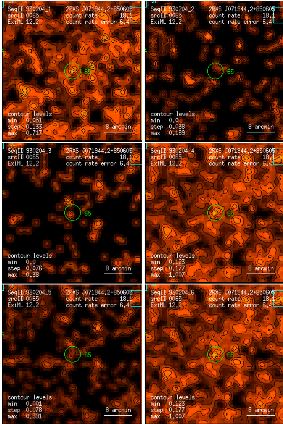
Figure 65: RASS 930204: detection 0065: band rate images, Gaussian filter: (1) PSPC channels 11 – 41, (2) 52 – 90, (3) 91 – 201, (4) 11 – 235, (5) 52 – 201, (6) 11 – 201. Broad band rates in counts/ks. Band rate contour levels in counts/ks/arcmin 2 .
