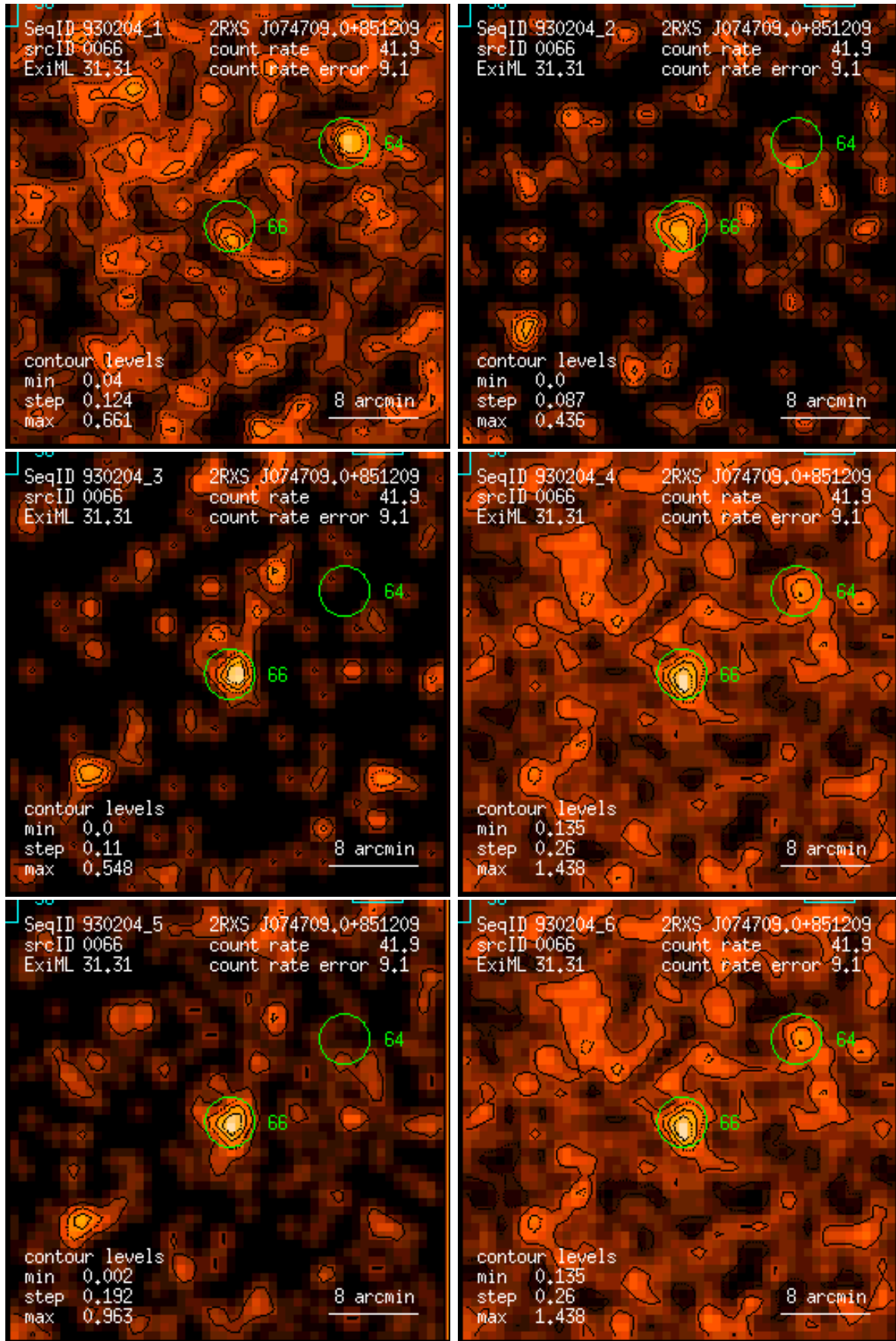
Figure 66: RASS 930204: detection 0066: band rate images, Gaussian filter: (1) PSPC channels 11 – 41, (2) 52 – 90, (3) 91 – 201, (4) 11 – 235, (5) 52 – 201, (6) 11 – 201. Broad band rates in counts/ks. Band rate contour levels in counts/ks/arcmin 2 .
