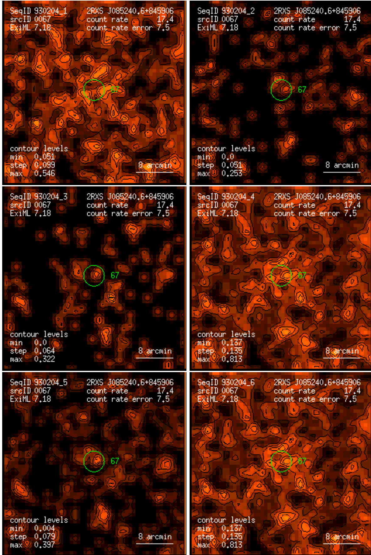
Figure 67: RASS 930204: detection 0067: band rate images, Gaussian filter: (1) PSPC channels 11 – 41, (2) 52 – 90, (3) 91 – 201, (4) 11 – 235, (5) 52 – 201, (6) 11 – 201. Broad band rates in counts/ks. Band rate contour levels in counts/ks/arcmin 2 .
