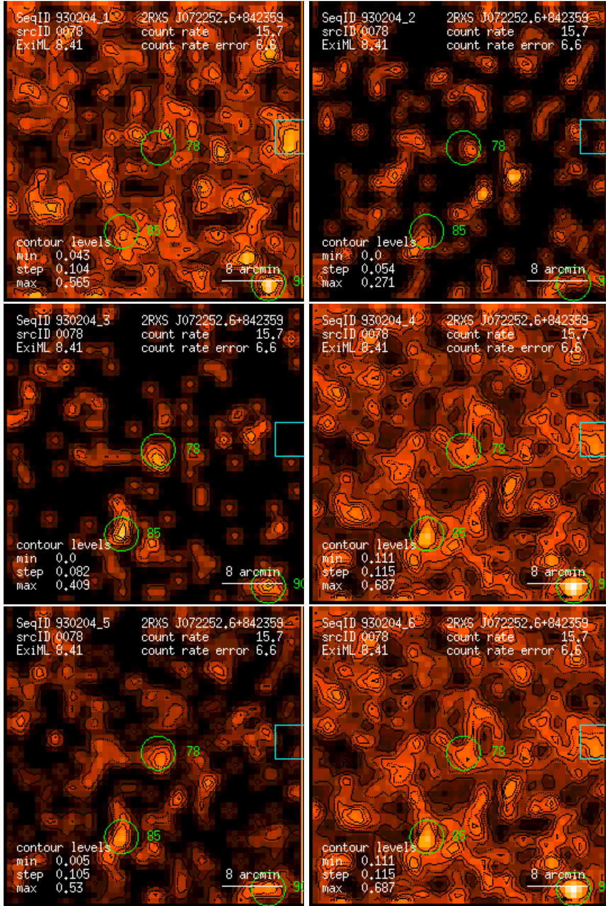
Figure 78: RASS 930204: detection 0078: band rate images, Gaussian filter: (1) PSPC channels 11 – 41, (2) 52 – 90, (3) 91 – 201, (4) 11 – 235, (5) 52 – 201, (6) 11 – 201. Broad band rates in counts/ks. Band rate contour levels in counts/ks/arcmin 2 .
