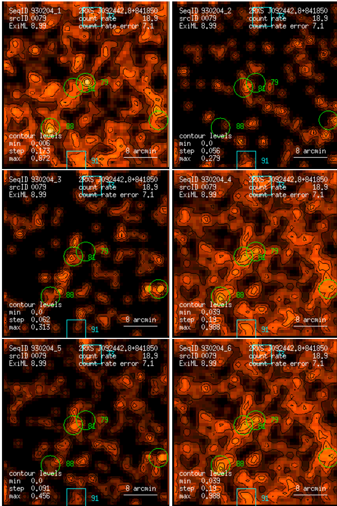
Figure 79: RASS 930204: detection 0079: band rate images, Gaussian filter: (1) PSPC channels 11 – 41, (2) 52 – 90, (3) 91 – 201, (4) 11 – 235, (5) 52 – 201, (6) 11 – 201. Broad band rates in counts/ks. Band rate contour levels in counts/ks/arcmin 2 .
