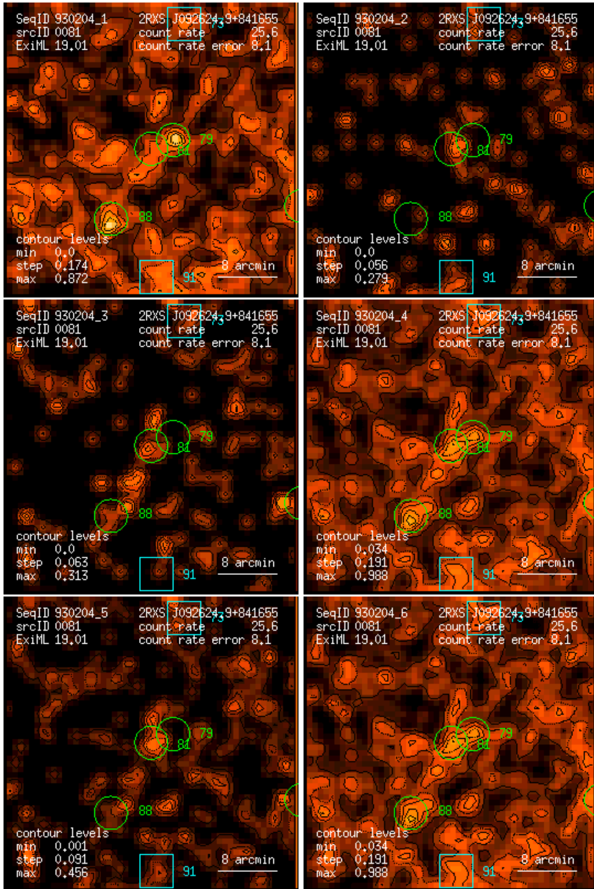
Figure 81: RASS 930204: detection 0081: band rate images, Gaussian filter: (1) PSPC channels 11 – 41, (2) 52 – 90, (3) 91 – 201, (4) 11 – 235, (5) 52 – 201, (6) 11 – 201. Broad band rates in counts/ks. Band rate contour levels in counts/ks/arcmin 2 .
