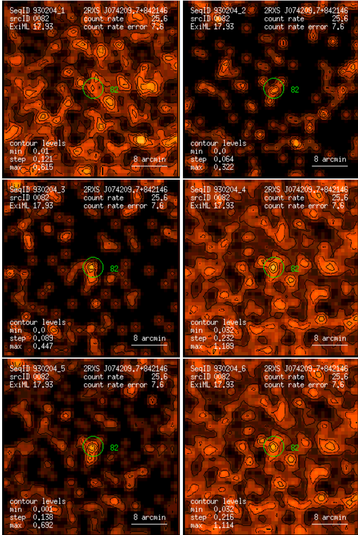
Figure 82: RASS 930204: detection 0082: band rate images, Gaussian filter: (1) PSPC channels 11 – 41, (2) 52 – 90, (3) 91 – 201, (4) 11 – 235, (5) 52 – 201, (6) 11 – 201. Broad band rates in counts/ks. Band rate contour levels in counts/ks/arcmin 2 .
