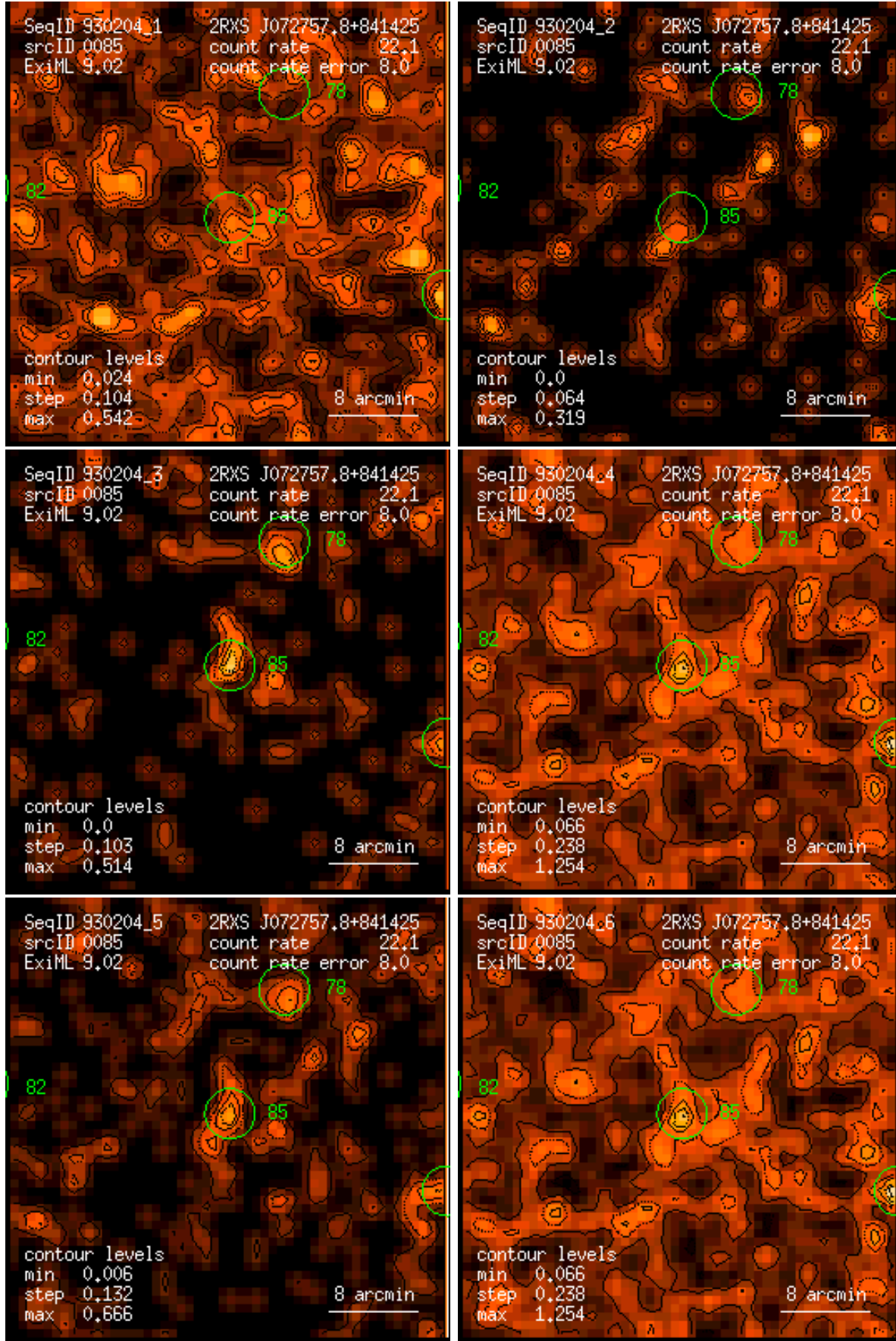
Figure 85: RASS 930204: detection 0085: band rate images, Gaussian filter: (1) PSPC channels 11 – 41, (2) 52 – 90, (3) 91 – 201, (4) 11 – 235, (5) 52 – 201, (6) 11 – 201. Broad band rates in counts/ks. Band rate contour levels in counts/ks/arcmin 2 .
