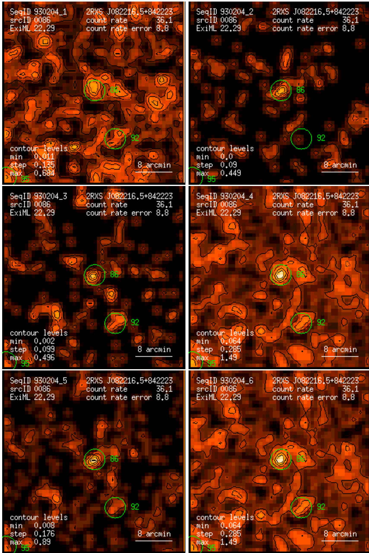
Figure 86: RASS 930204: detection 0086: band rate images, Gaussian filter: (1) PSPC channels 11 – 41, (2) 52 – 90, (3) 91 – 201, (4) 11 – 235, (5) 52 – 201, (6) 11 – 201. Broad band rates in counts/ks. Band rate contour levels in counts/ks/arcmin 2 .
