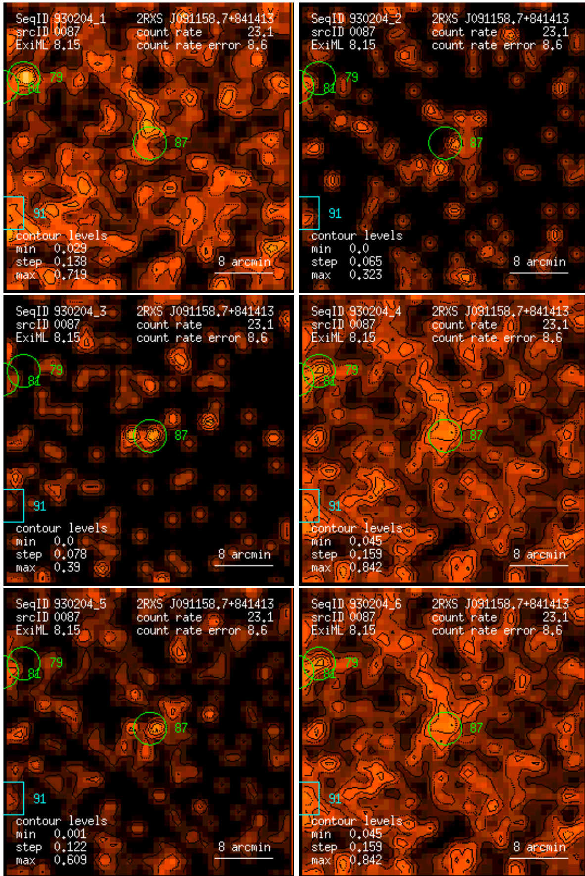
Figure 87: RASS 930204: detection 0087: band rate images, Gaussian filter: (1) PSPC channels 11 – 41, (2) 52 – 90, (3) 91 – 201, (4) 11 – 235, (5) 52 – 201, (6) 11 – 201. Broad band rates in counts/ks. Band rate contour levels in counts/ks/arcmin 2 .
