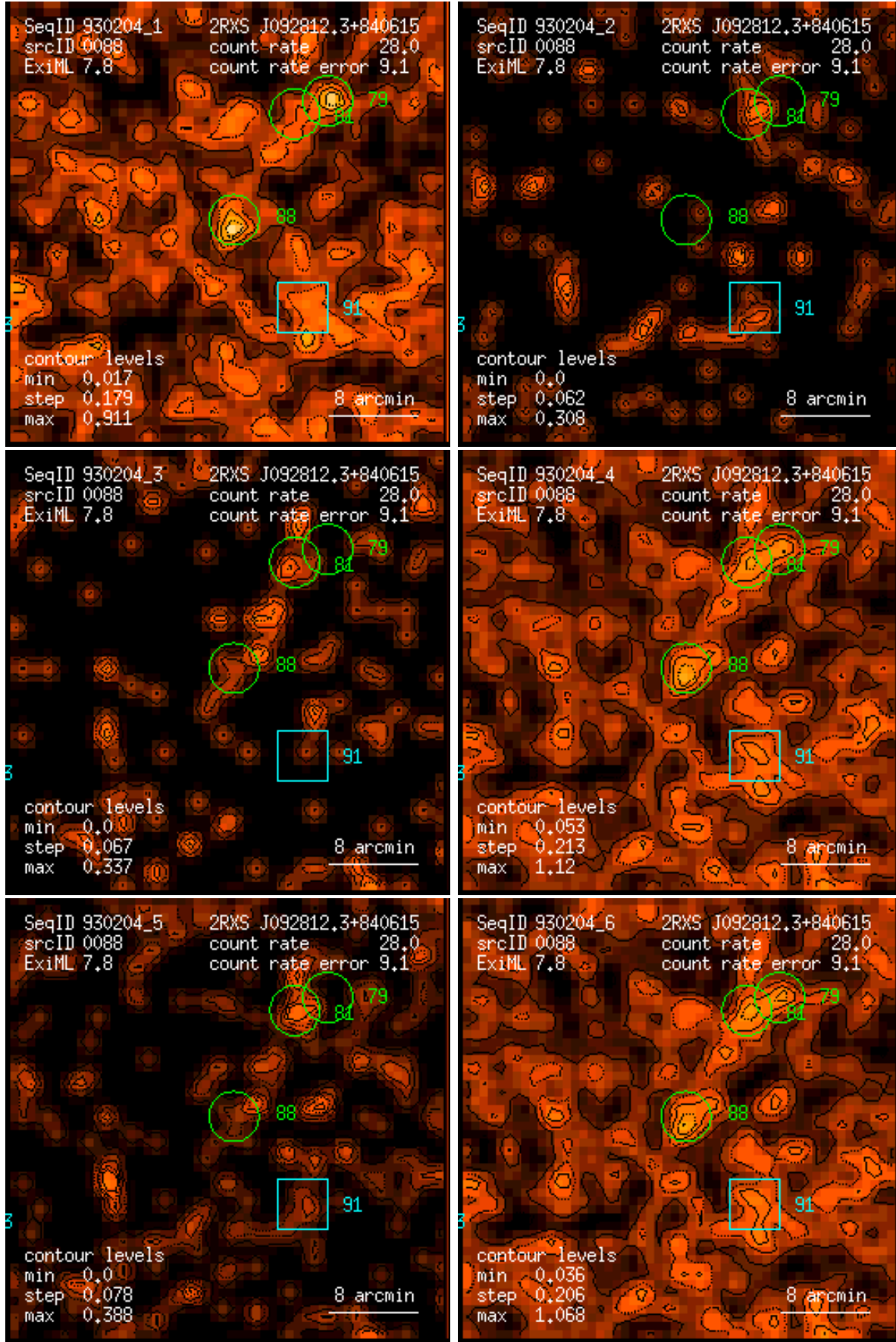
Figure 88: RASS 930204: detection 0088: band rate images, Gaussian filter: (1) PSPC channels 11 – 41, (2) 52 – 90, (3) 91 – 201, (4) 11 – 235, (5) 52 – 201, (6) 11 – 201. Broad band rates in counts/ks. Band rate contour levels in counts/ks/arcmin 2 .
