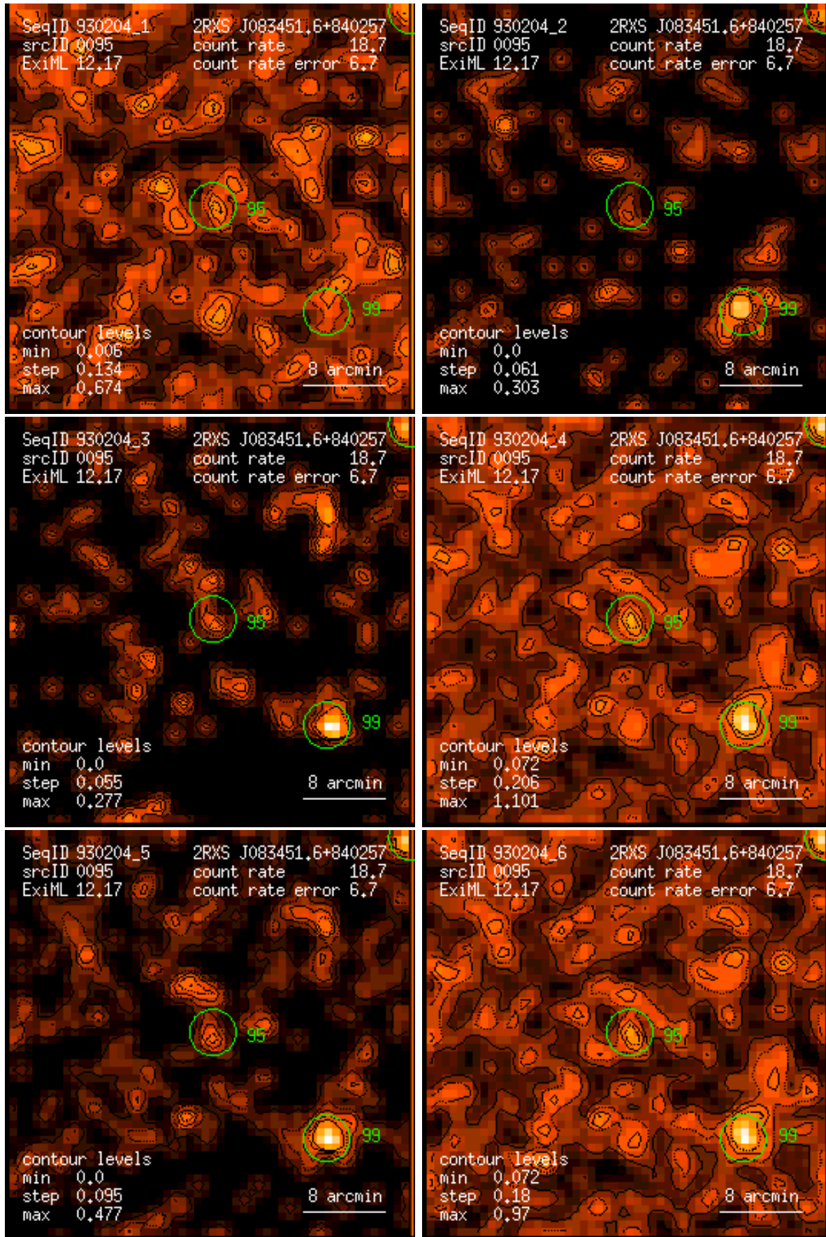
Figure 95: RASS 930204: detection 0095: band rate images, Gaussian filter: (1) PSPC channels 11 – 41, (2) 52 – 90, (3) 91 – 201, (4) 11 – 235, (5) 52 – 201, (6) 11 – 201. Broad band rates in counts/ks. Band rate contour levels in counts/ks/arcmin 2 .
