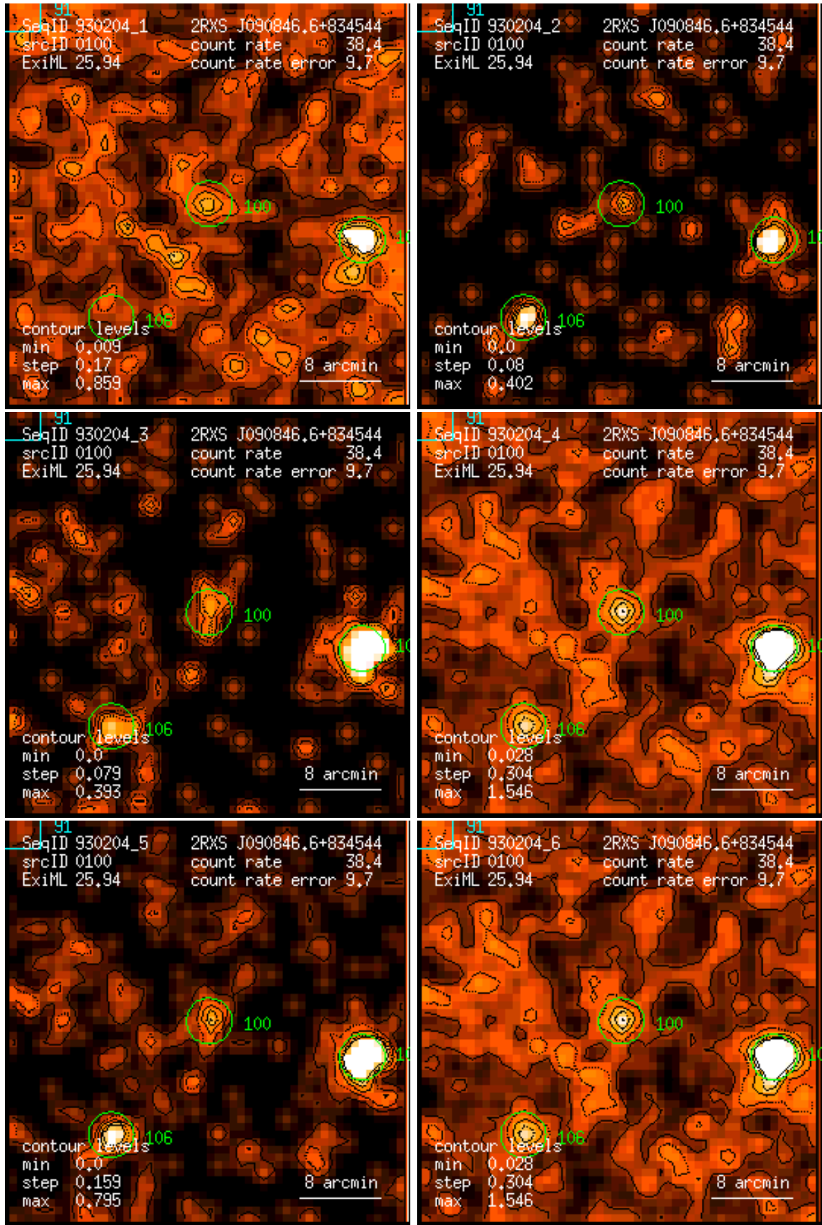
Figure 100: RASS 930204: detection 0100: band rate images, Gaussian filter: (1) PSPC channels 11 – 41, (2) 52 – 90, (3) 91 – 201, (4) 11 – 235, (5) 52 – 201, (6) 11 – 201. Broad band rates in counts/ks. Band rate contour levels in counts/ks/arcmin 2 .
