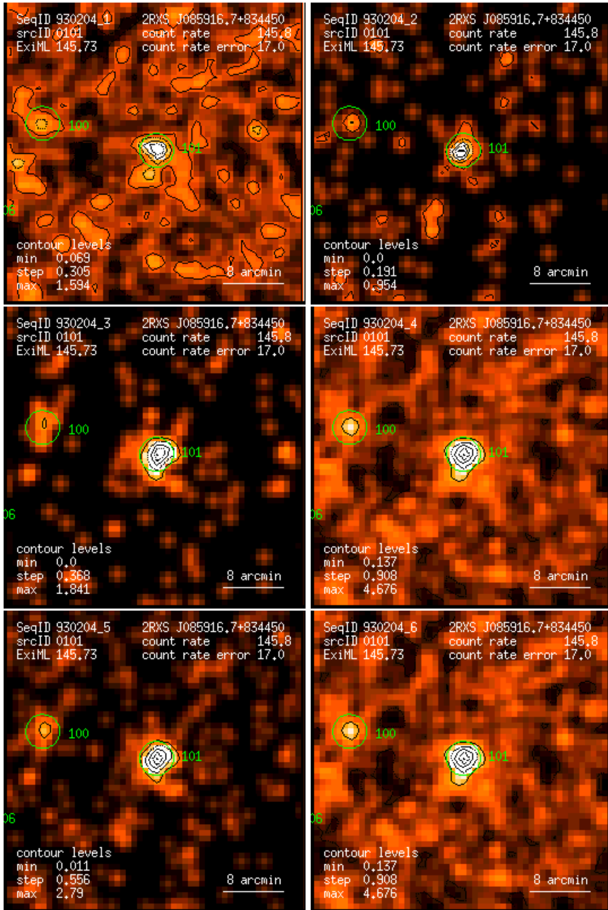
Figure 101: RASS 930204: detection 0101: band rate images, Gaussian filter: (1) PSPC channels 11 – 41, (2) 52 – 90, (3) 91 – 201, (4) 11 – 235, (5) 52 – 201, (6) 11 – 201. Broad band rates in counts/ks. Band rate contour levels in counts/ks/arcmin 2 .
