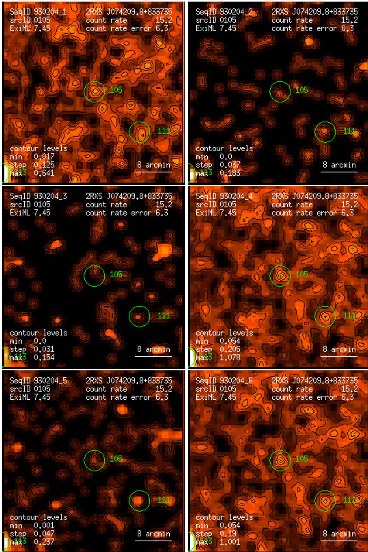
Figure 105: RASS 930204: detection 0105: band rate images, Gaussian filter: (1) PSPC channels 11 – 41, (2) 52 – 90, (3) 91 – 201, (4) 11 – 235, (5) 52 – 201, (6) 11 – 201. Broad band rates in counts/ks. Band rate contour levels in counts/ks/arcmin 2 .
