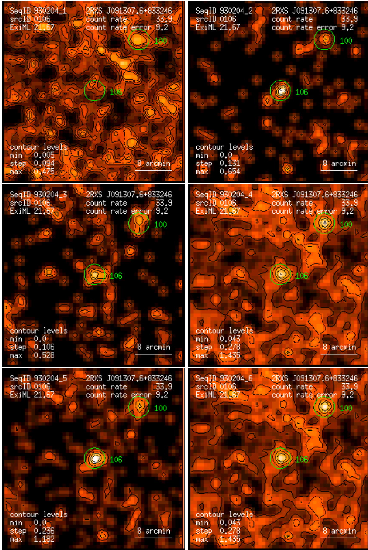
Figure 106: RASS 930204: detection 0106: band rate images, Gaussian filter: (1) PSPC channels 11 – 41, (2) 52 – 90, (3) 91 – 201, (4) 11 – 235, (5) 52 – 201, (6) 11 – 201. Broad band rates in counts/ks. Band rate contour levels in counts/ks/arcmin 2 .
