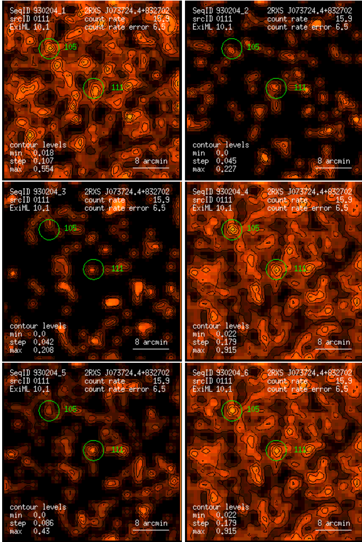
Figure 111: RASS 930204: detection 0111: band rate images, Gaussian filter: (1) PSPC channels 11 – 41, (2) 52 – 90, (3) 91 – 201, (4) 11 – 235, (5) 52 – 201, (6) 11 – 201. Broad band rates in counts/ks. Band rate contour levels in counts/ks/arcmin 2 .
