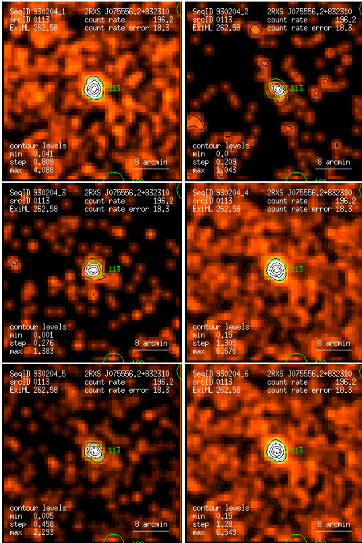
Figure 113: RASS 930204: detection 0113: band rate images, Gaussian filter: (1) PSPC channels 11 – 41, (2) 52 – 90, (3) 91 – 201, (4) 11 – 235, (5) 52 – 201, (6) 11 – 201. Broad band rates in counts/ks. Band rate contour levels in counts/ks/arcmin 2 .
