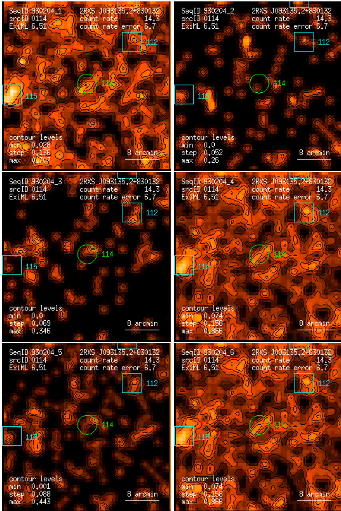
Figure 114: RASS 930204: detection 0114: band rate images, Gaussian filter: (1) PSPC channels 11 – 41, (2) 52 – 90, (3) 91 – 201, (4) 11 – 235, (5) 52 – 201, (6) 11 – 201. Broad band rates in counts/ks. Band rate contour levels in counts/ks/arcmin 2 .
