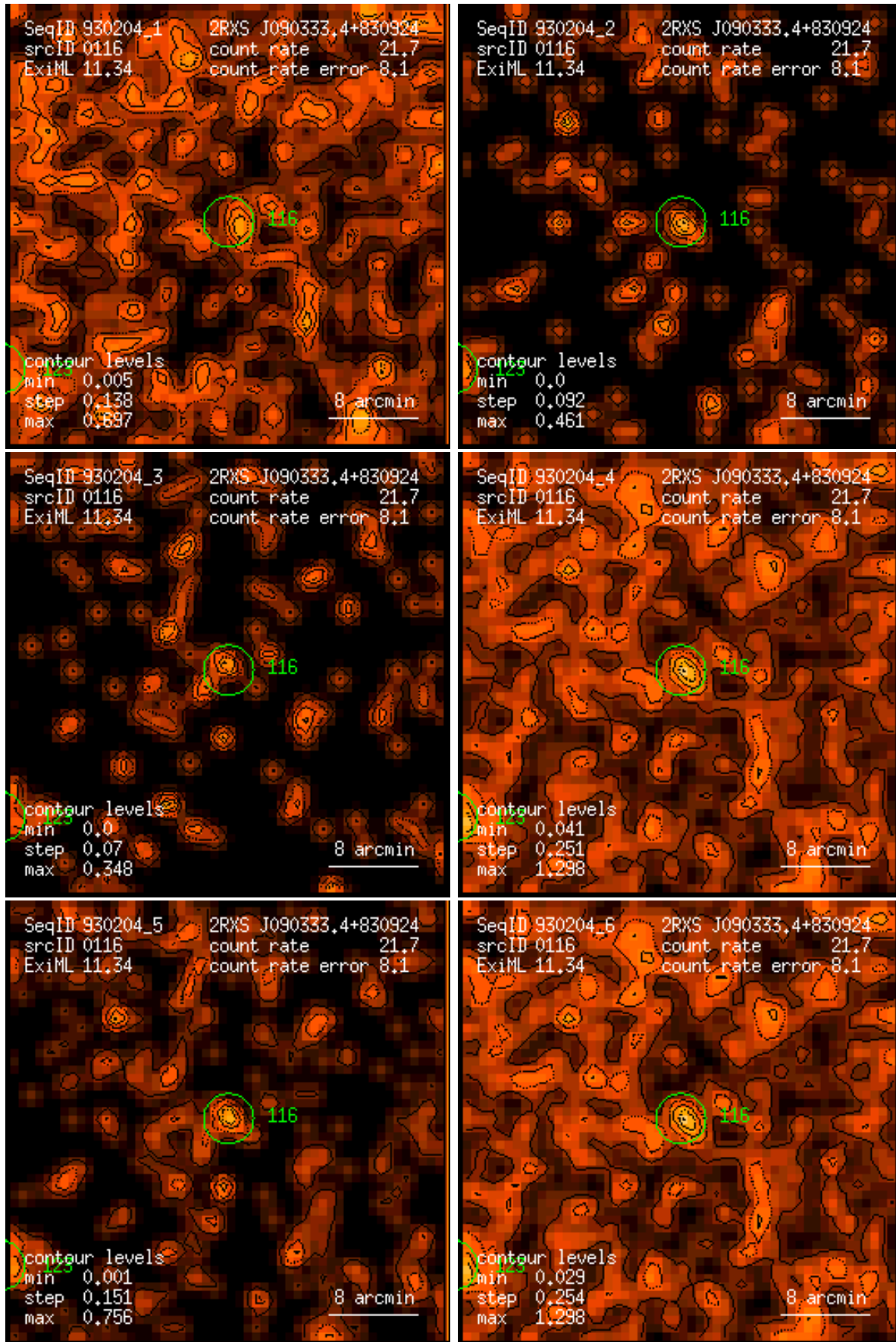
Figure 116: RASS 930204: detection 0116: band rate images, Gaussian filter: (1) PSPC channels 11 – 41, (2) 52 – 90, (3) 91 – 201, (4) 11 – 235, (5) 52 – 201, (6) 11 – 201. Broad band rates in counts/ks. Band rate contour levels in counts/ks/arcmin 2 .
