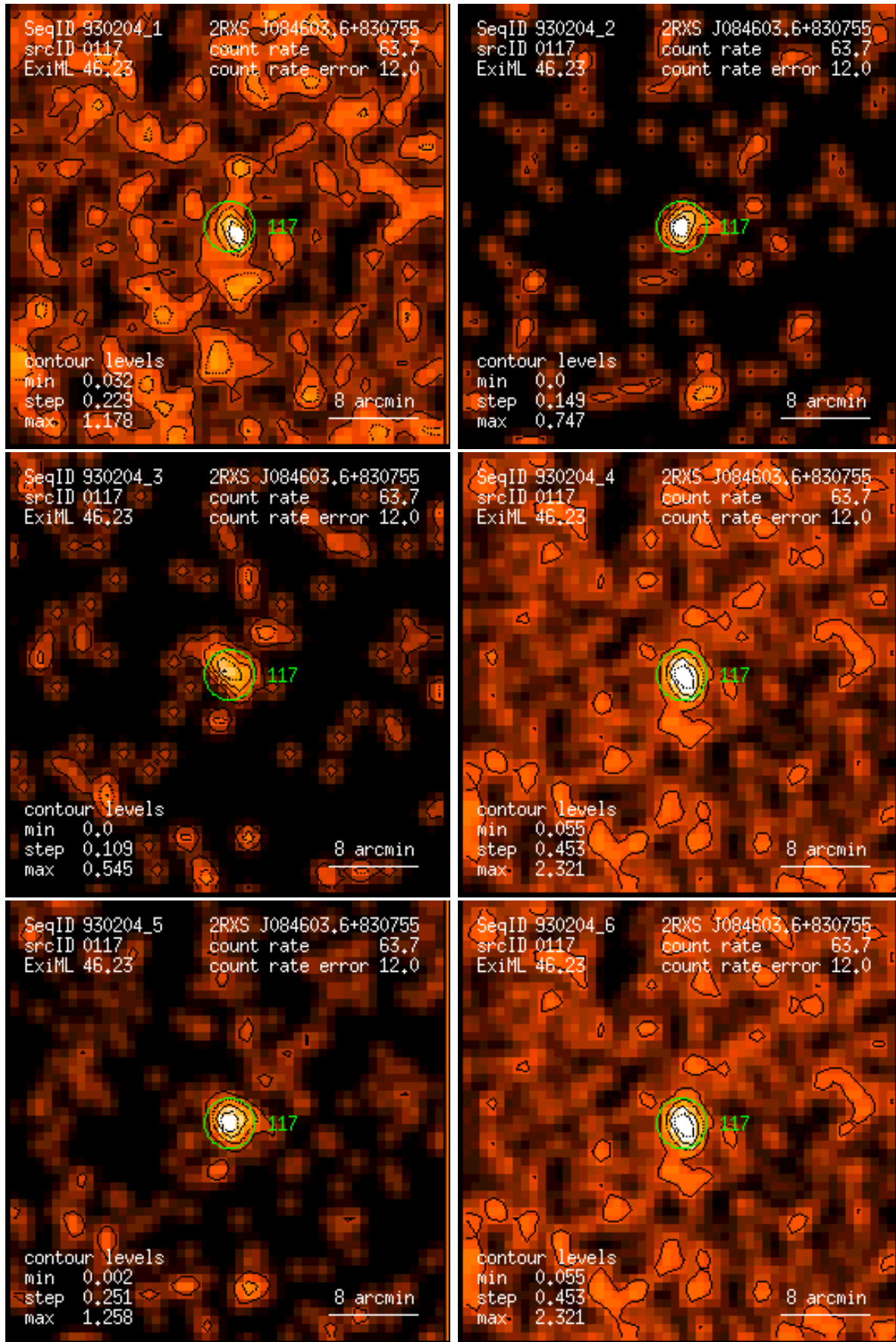
Figure 117: RASS 930204: detection 0117: band rate images, Gaussian filter: (1) PSPC channels 11 – 41, (2) 52 – 90, (3) 91 – 201, (4) 11 – 235, (5) 52 – 201, (6) 11 – 201. Broad band rates in counts/ks. Band rate contour levels in counts/ks/arcmin 2 .
