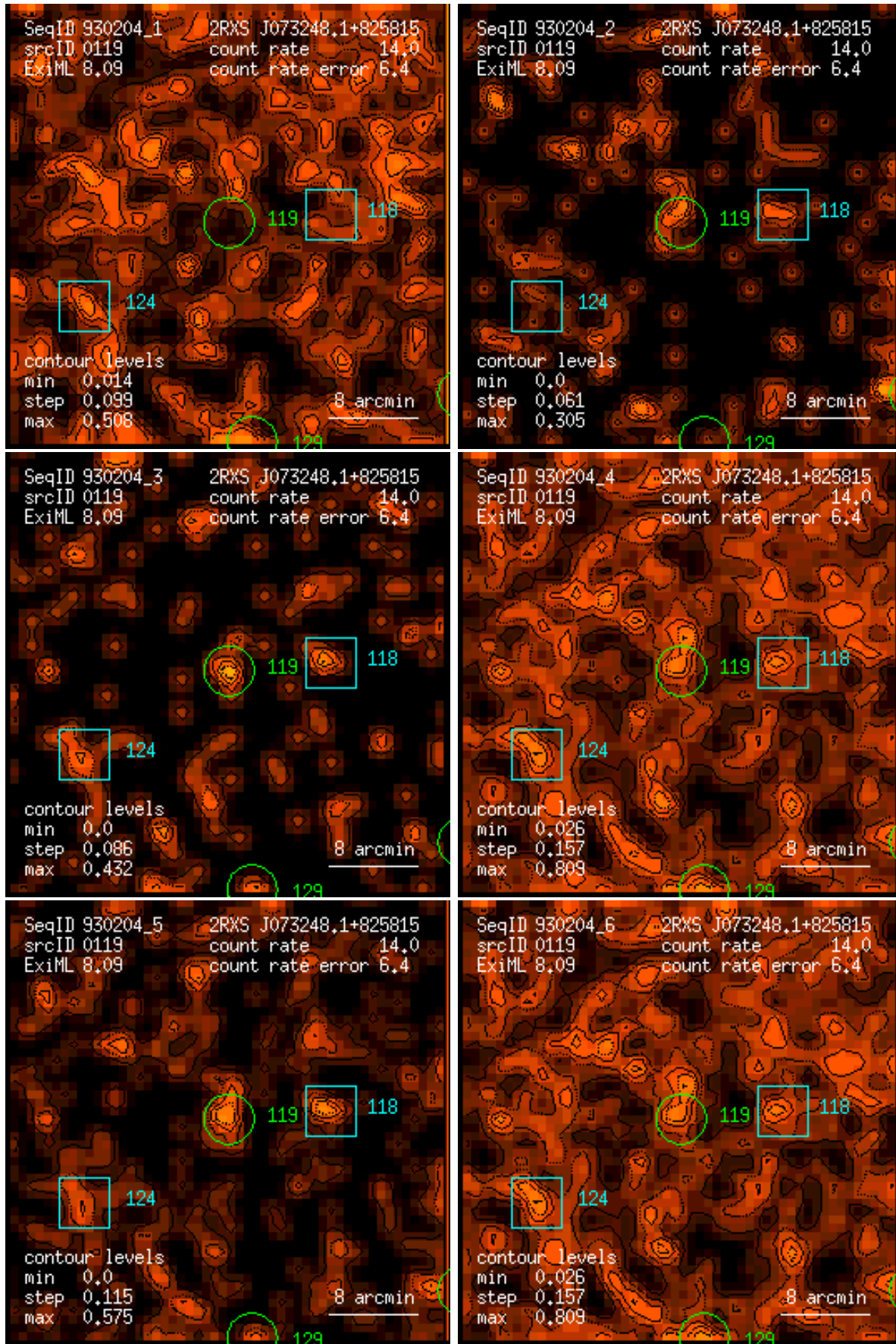
Figure 119: RASS 930204: detection 0119: band rate images, Gaussian filter: (1) PSPC channels 11 – 41, (2) 52 – 90, (3) 91 – 201, (4) 11 – 235, (5) 52 – 201, (6) 11 – 201. Broad band rates in counts/ks. Band rate contour levels in counts/ks/arcmin 2 .
